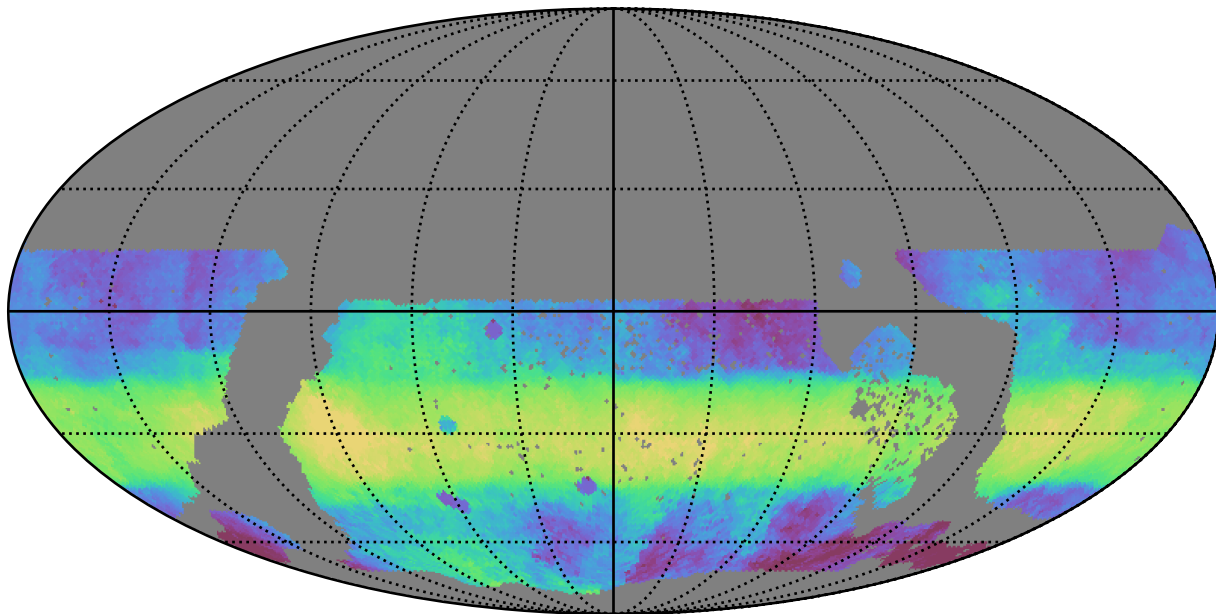
early_ss_template_fpextra2.0_v3.4_10yrs WFD i band: Median HA
