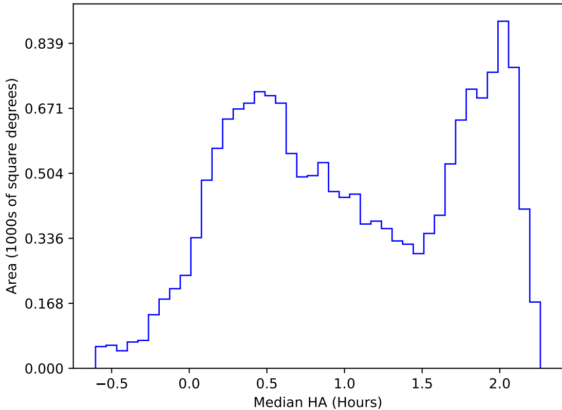
early_ss_template_fpextra2.0_v3.4_10yrs WFD i band: Median HA
