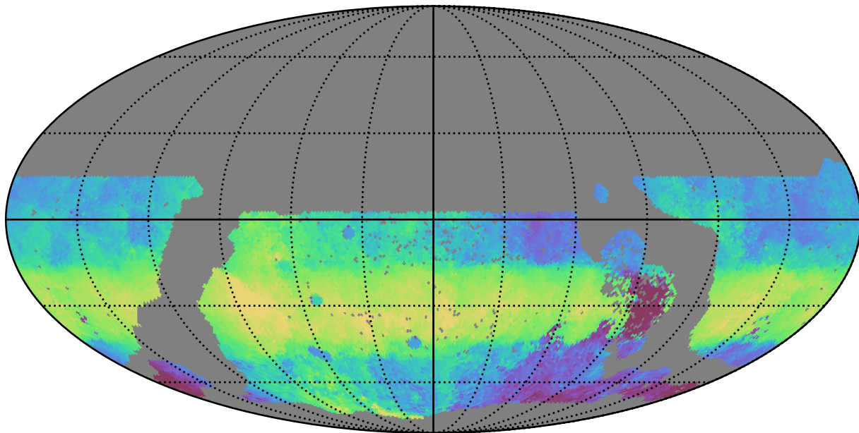
early_ss_template_fpextra2.0_v3.4_10yrs WFD g band: Median HA
