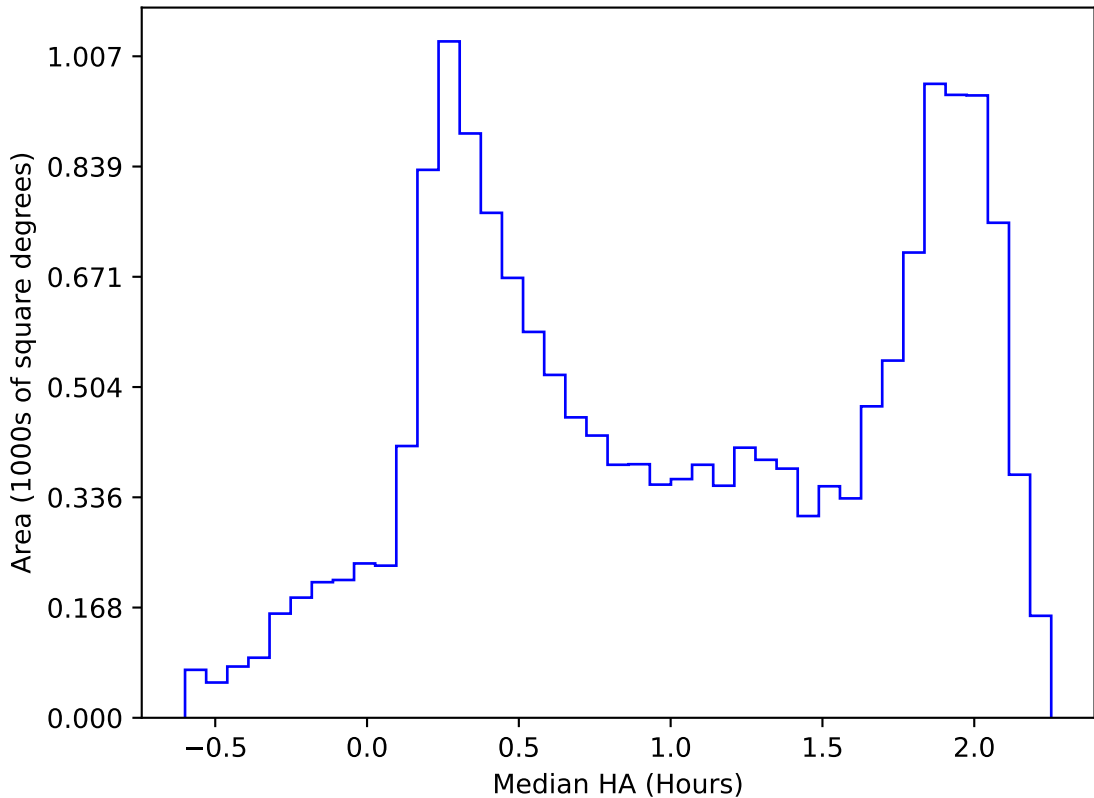
early_ss_template_fpextra2.0_v3.4_10yrs WFD all bands: Median HA
