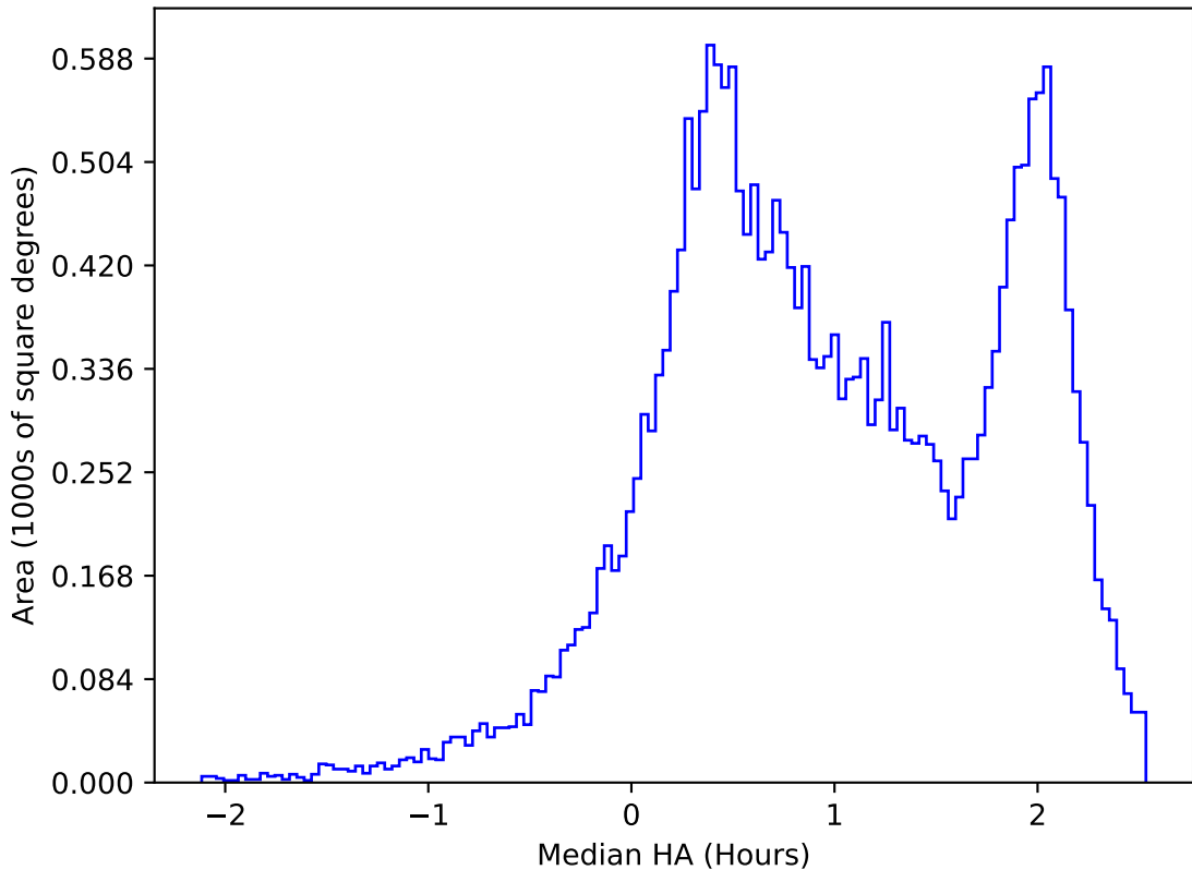
early_ss_template_fpextra2.0_v3.4_10yrs All sky z band: Median HA
