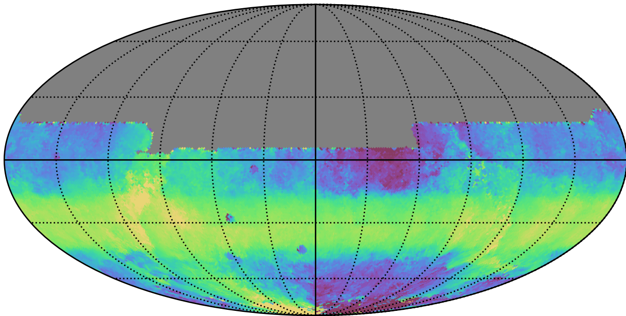
early_ss_template_fpextra2.0_v3.4_10yrs All sky y band: Median HA
