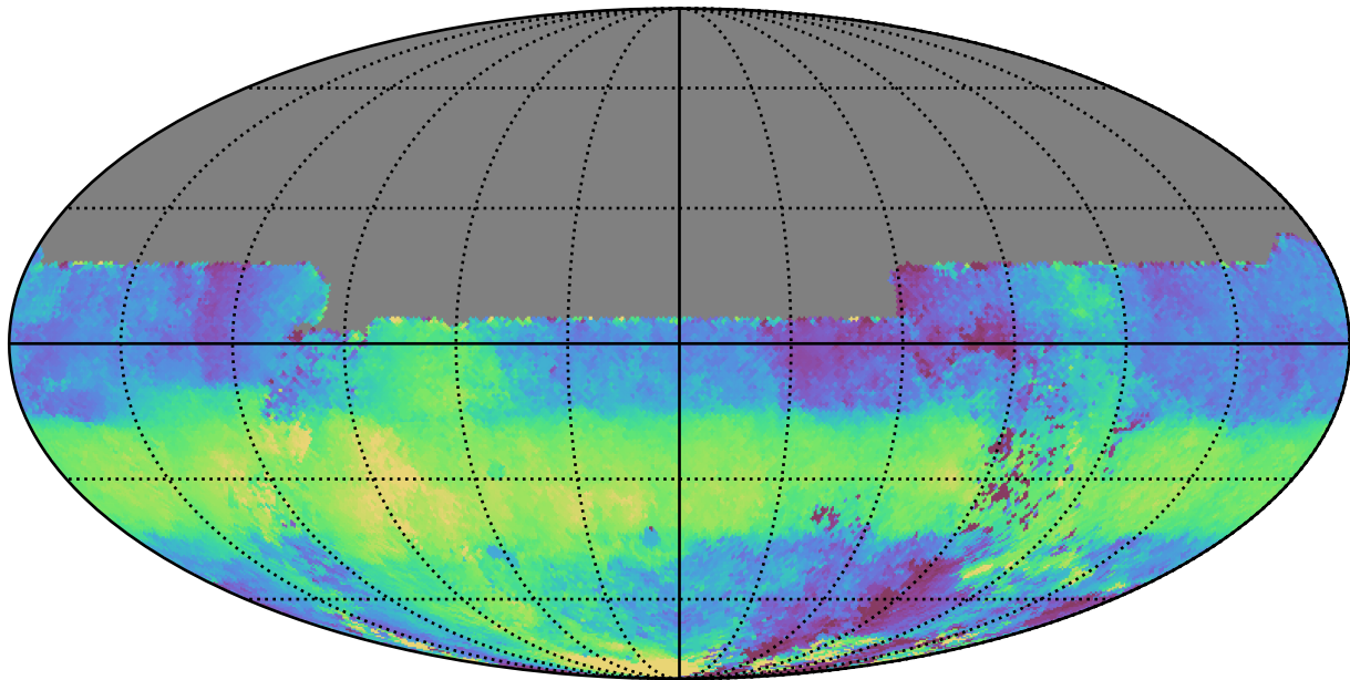
early_ss_template_fpextra2.0_v3.4_10yrs All sky u band: Median HA
