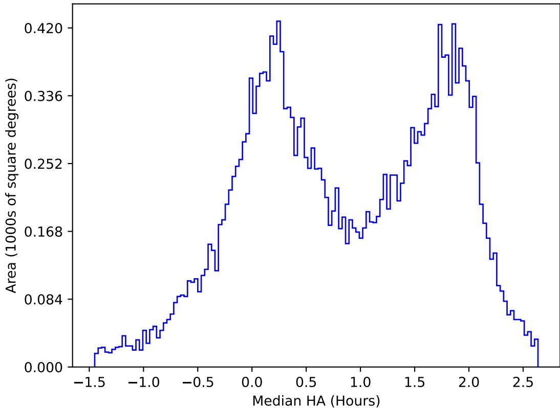
early_ss_template_fpextra2.0_v3.4_10yrs All sky u band: Median HA
