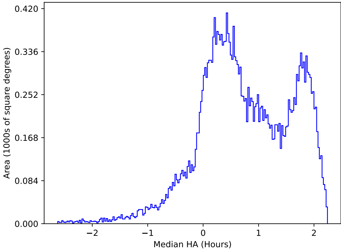
early_ss_template_fpextra2.0_v3.4_10yrs All sky r band: Median HA
