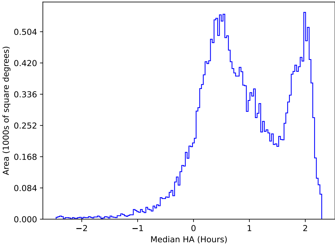
early_ss_template_fpextra2.0_v3.4_10yrs All sky i band: Median HA
