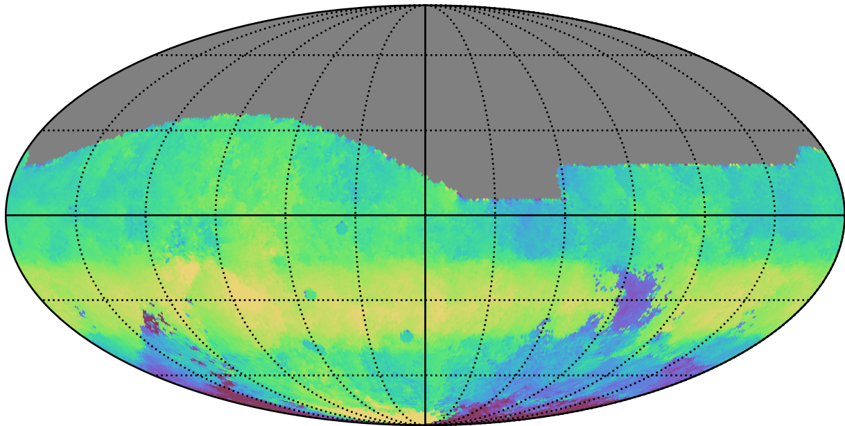
early_ss_template_fpextra2.0_v3.4_10yrs All sky g band: Median HA
