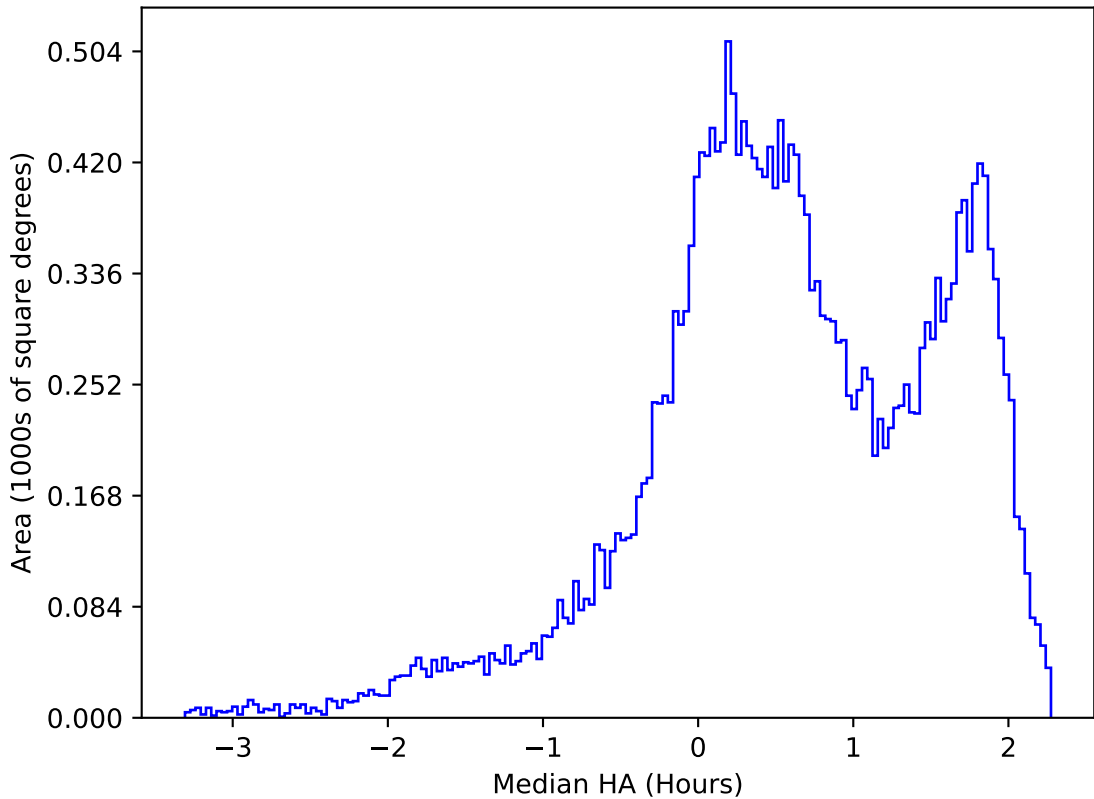
early_ss_template_fpextra2.0_v3.4_10yrs All sky g band: Median HA
