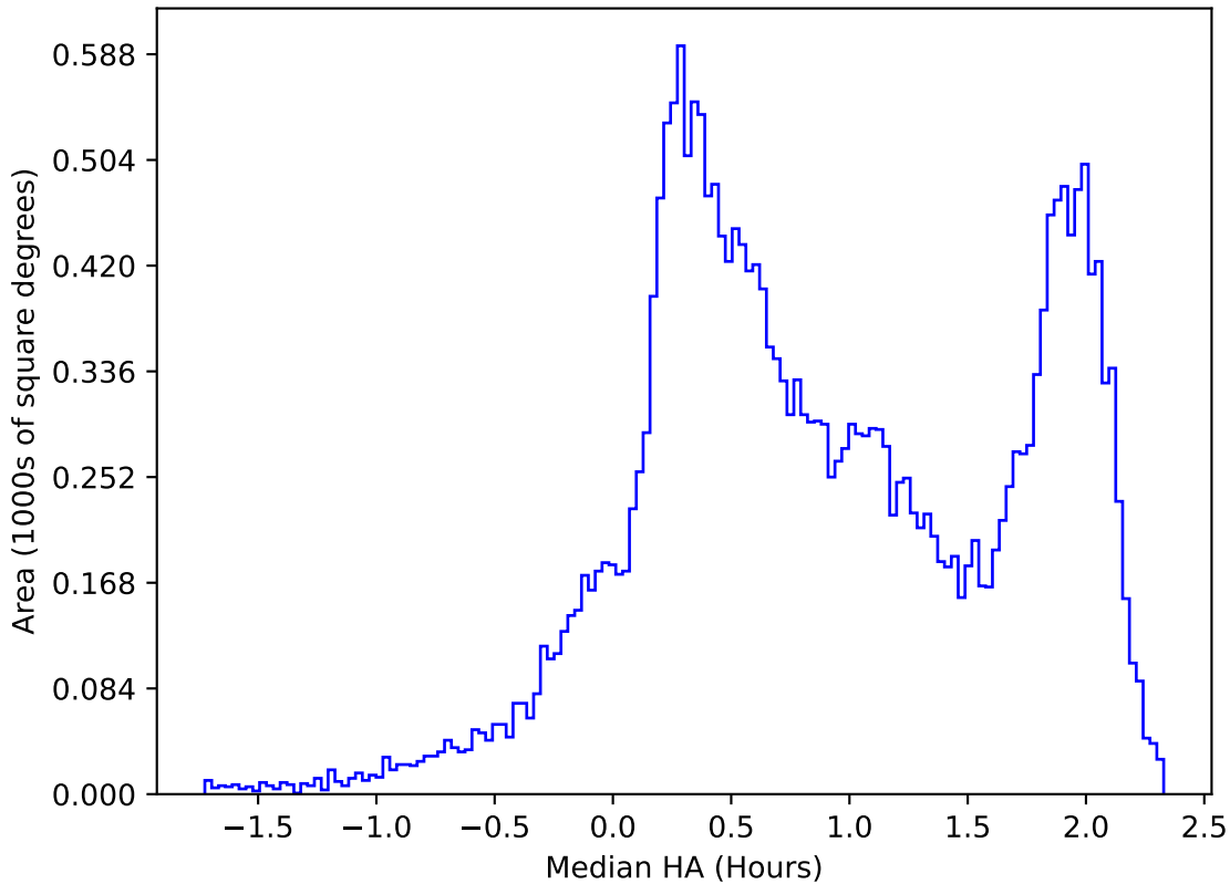
early_ss_template_fpextra2.0_v3.4_10yrs All sky all bands: Median HA
