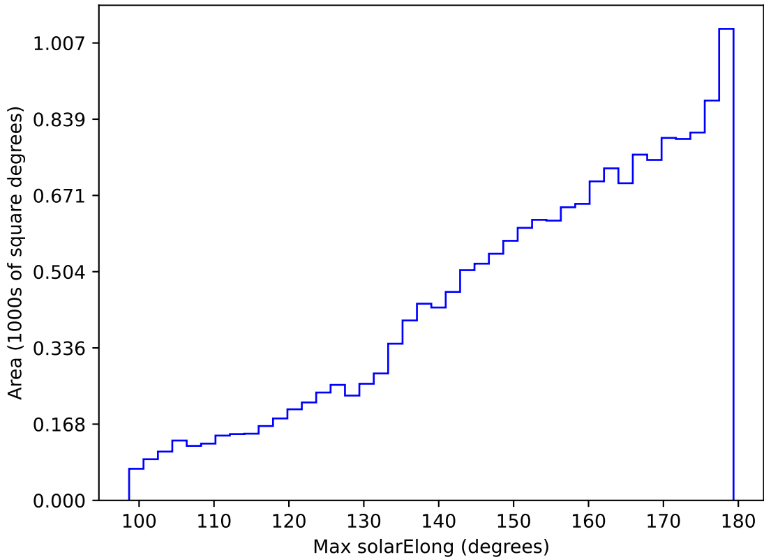
early_ss_template_fpextra2.0_v3.4_10yrs WFD z band: Max solarElong
