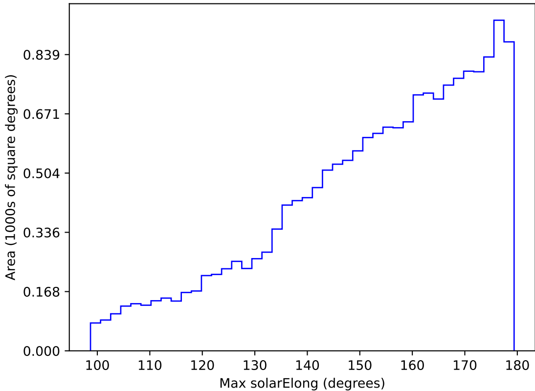
early_ss_template_fpextra2.0_v3.4_10yrs WFD y band: Max solarElong
