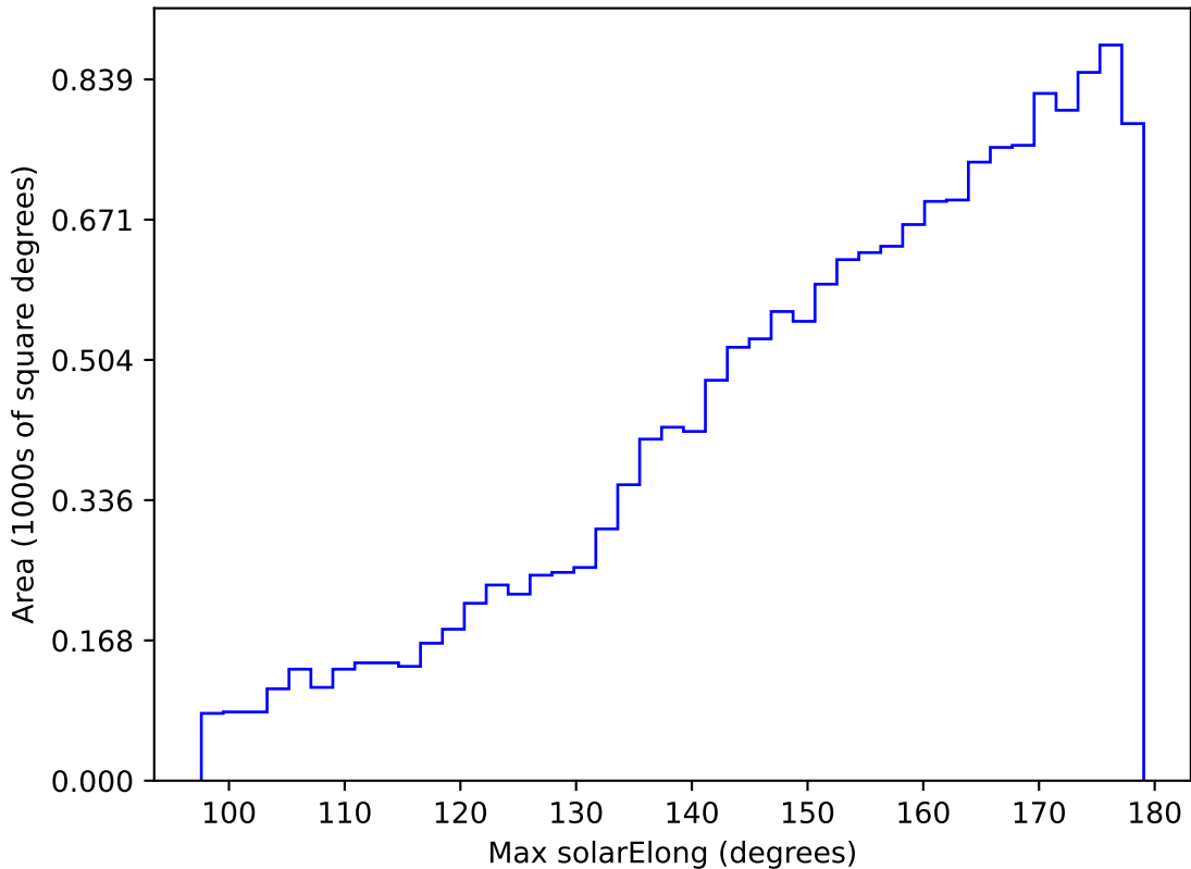
early_ss_template_fpextra2.0_v3.4_10yrs WFD u band: Max solarElong
