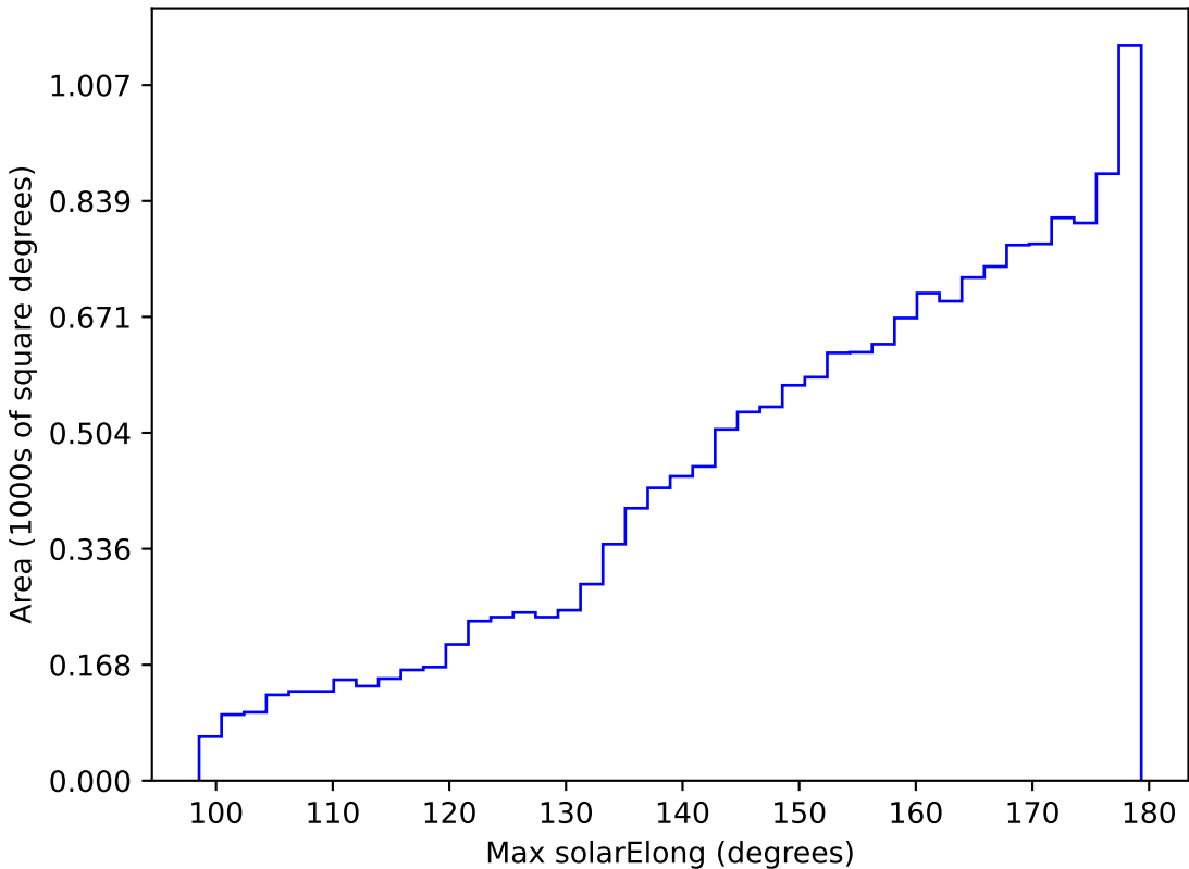
early_ss_template_fpextra2.0_v3.4_10yrs WFD r band: Max solarElong
