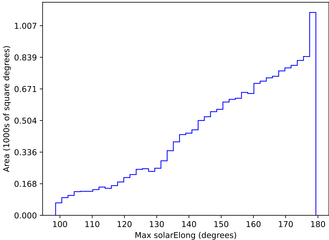
early_ss_template_fpextra2.0_v3.4_10yrs WFD i band: Max solarElong
