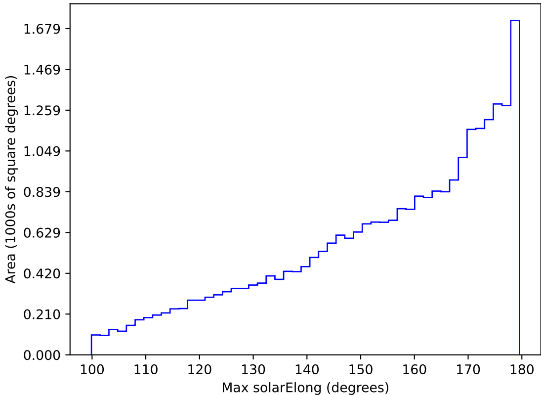
early_ss_template_fpextra2.0_v3.4_10yrs All sky all bands: Max solarElong
