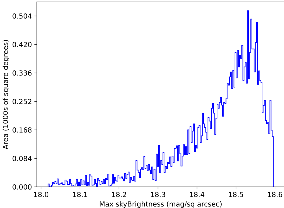
early_ss_template_fpextra2.0_v3.4_10yrs Yr 1 y band: Max skyBrightness
