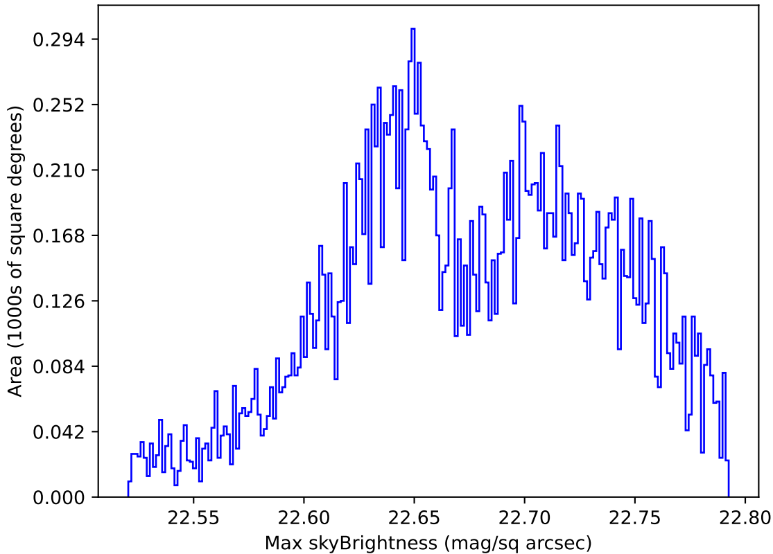
early_ss_template_fpextra2.0_v3.4_10yrs Yr 1 u band: Max skyBrightness
