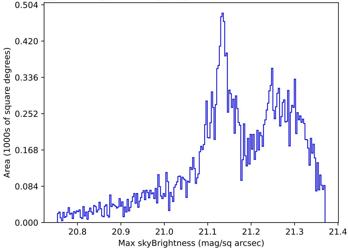
early_ss_template_fpextra2.0_v3.4_10yrs Yr 1 r band: Max skyBrightness
