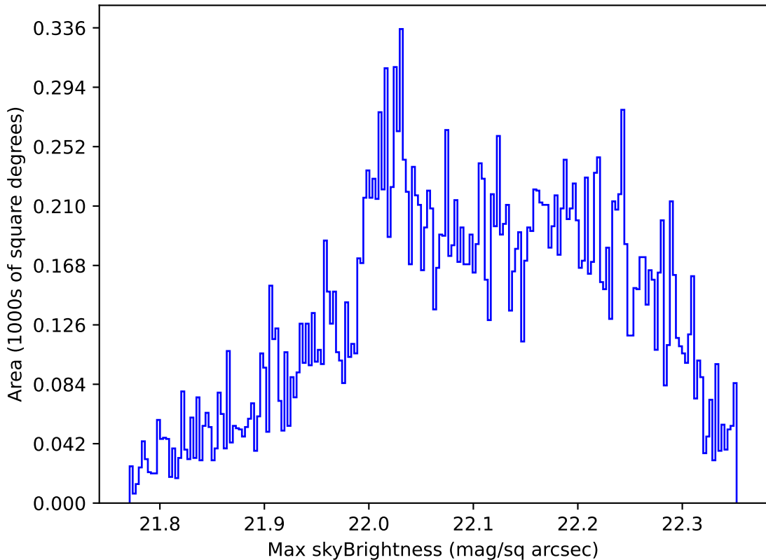
early_ss_template_fpextra2.0_v3.4_10yrs Yr 1 g band: Max skyBrightness
