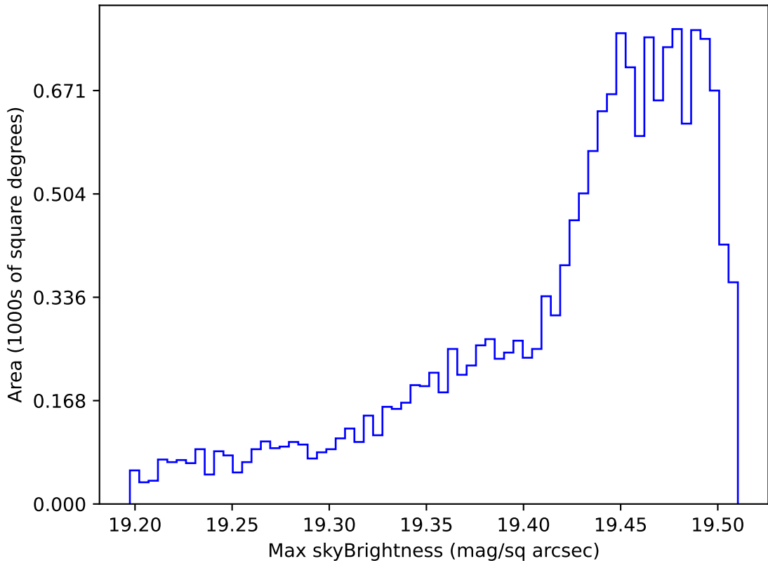
early_ss_template_fpextra2.0_v3.4_10yrs WFD z band: Max skyBrightness
