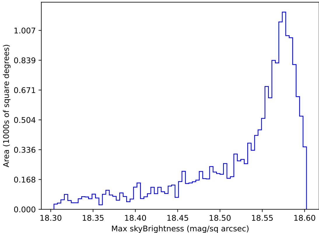
early_ss_template_fpextra2.0_v3.4_10yrs WFD y band: Max skyBrightness
