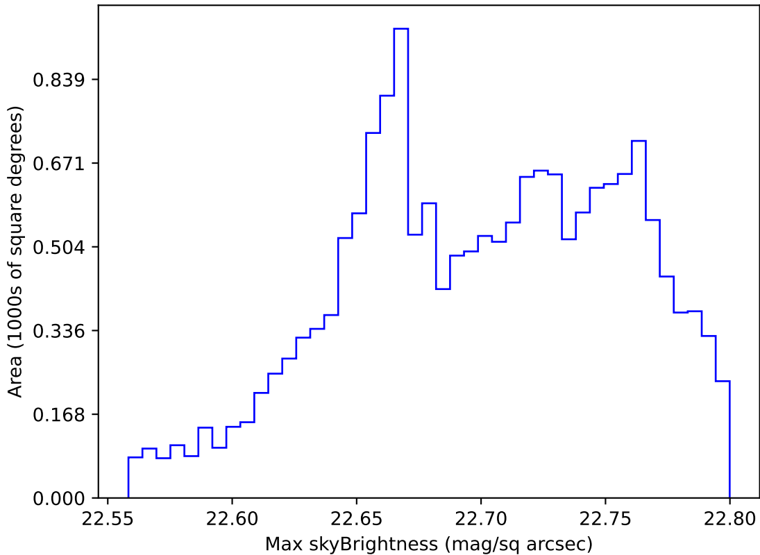
early_ss_template_fpextra2.0_v3.4_10yrs WFD u band: Max skyBrightness
