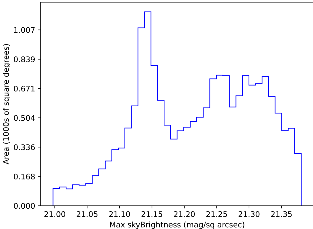
early_ss_template_fpextra2.0_v3.4_10yrs WFD r band: Max skyBrightness
