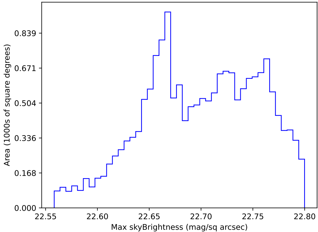
early_ss_template_fpextra2.0_v3.4_10yrs WFD all bands: Max skyBrightness
