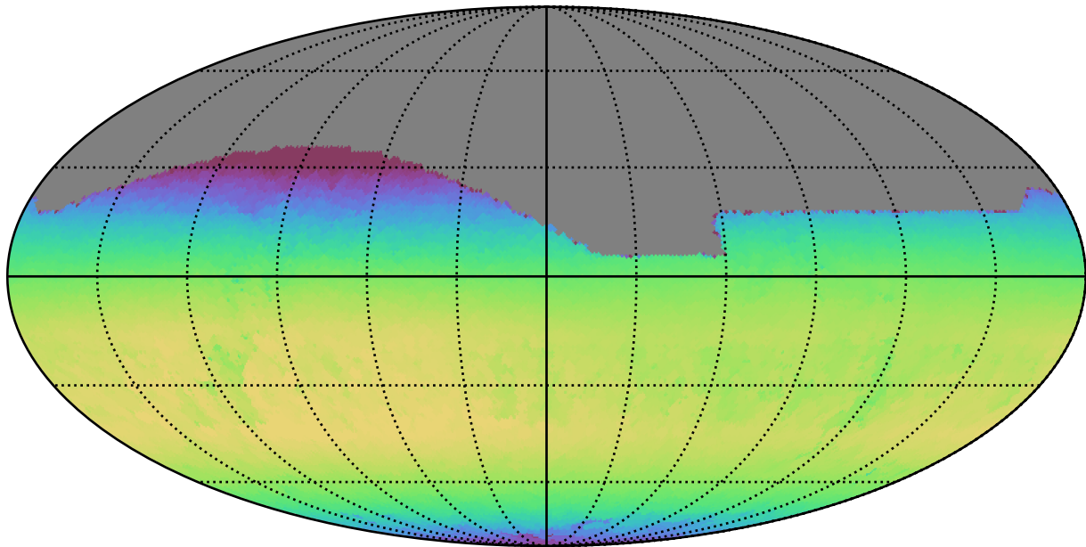
early_ss_template_fpextra2.0_v3.4_10yrs All sky z band: Max skyBrightness
