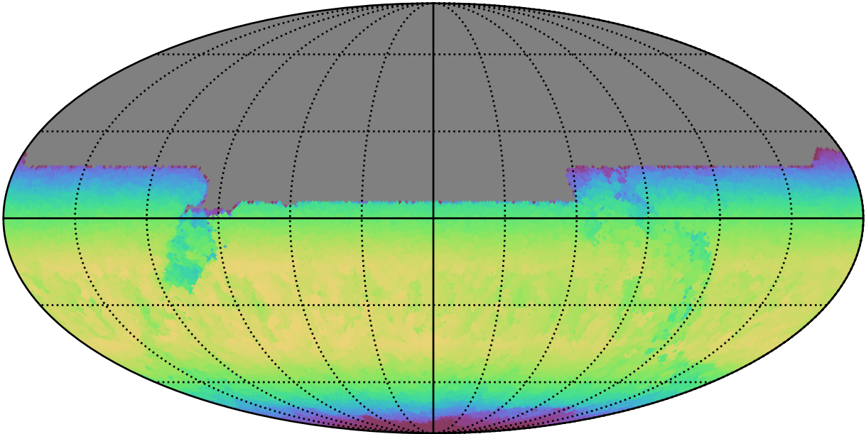
early_ss_template_fpextra2.0_v3.4_10yrs All sky y band: Max skyBrightness
