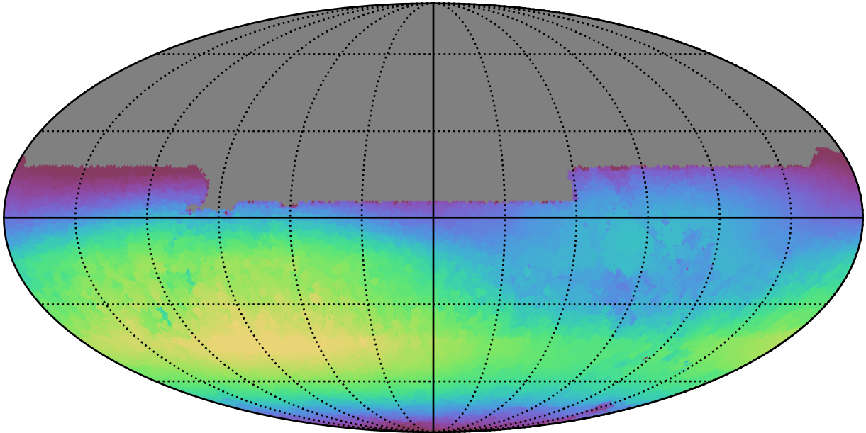
early_ss_template_fpextra2.0_v3.4_10yrs All sky u band: Max skyBrightness
