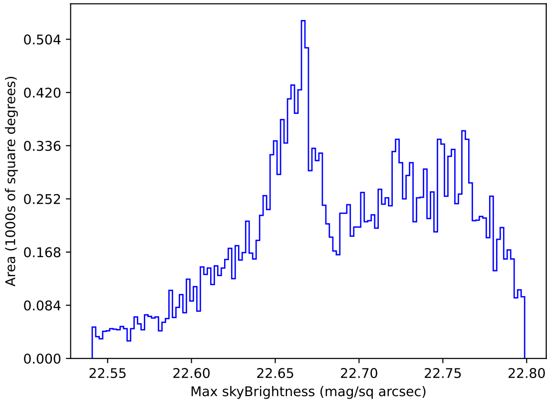
early_ss_template_fpextra2.0_v3.4_10yrs All sky u band: Max skyBrightness
