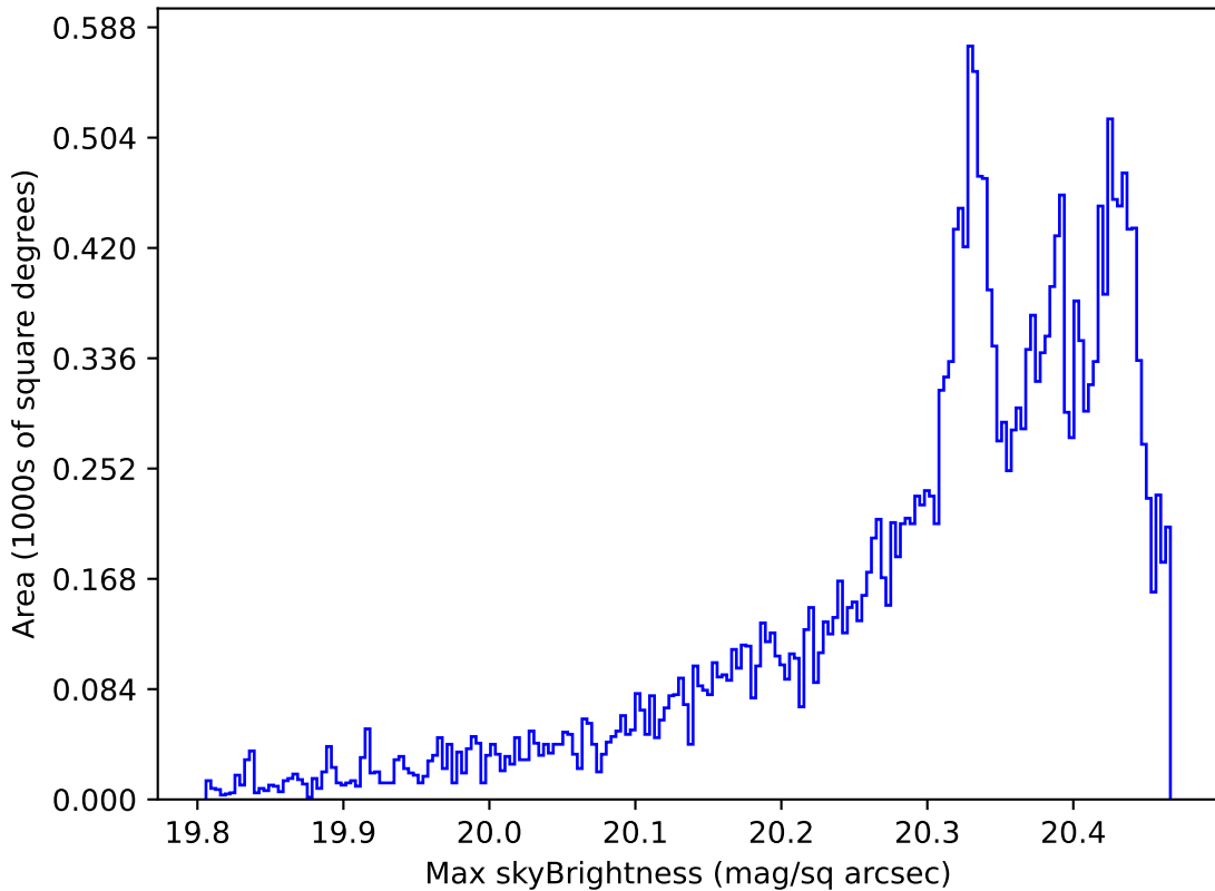
early_ss_template_fpextra2.0_v3.4_10yrs All sky i band: Max skyBrightness
