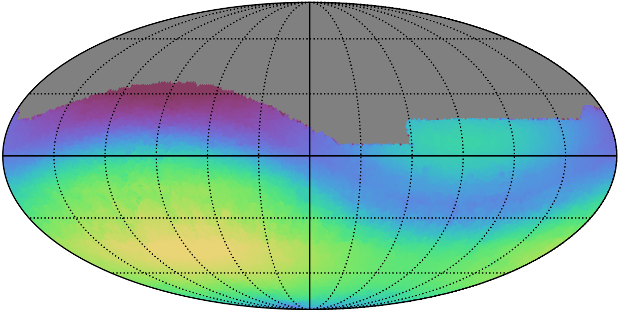
early_ss_template_fpextra2.0_v3.4_10yrs All sky g band: Max skyBrightness
