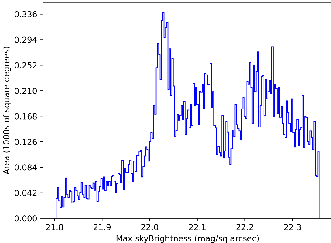
early_ss_template_fpextra2.0_v3.4_10yrs All sky g band: Max skyBrightness
