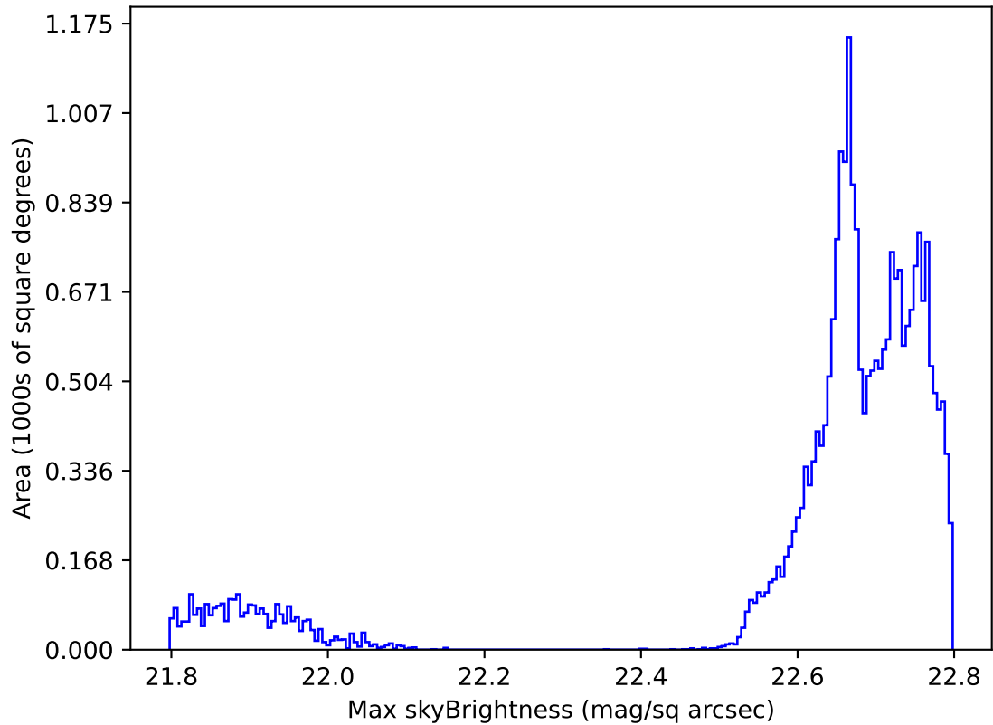
early_ss_template_fpextra2.0_v3.4_10yrs All sky all bands: Max skyBrightness
