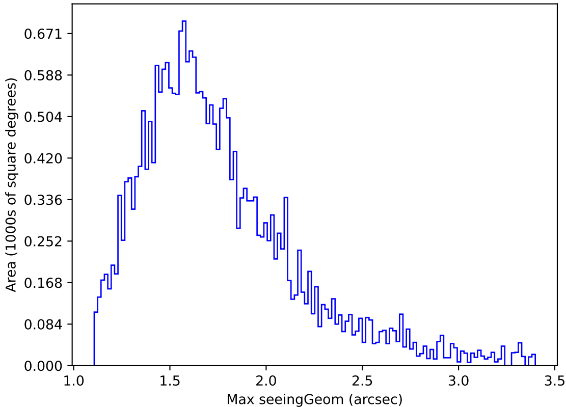
early_ss_template_fpextra2.0_v3.4_10yrs Yr 1 all bands: Max seeingGeom
