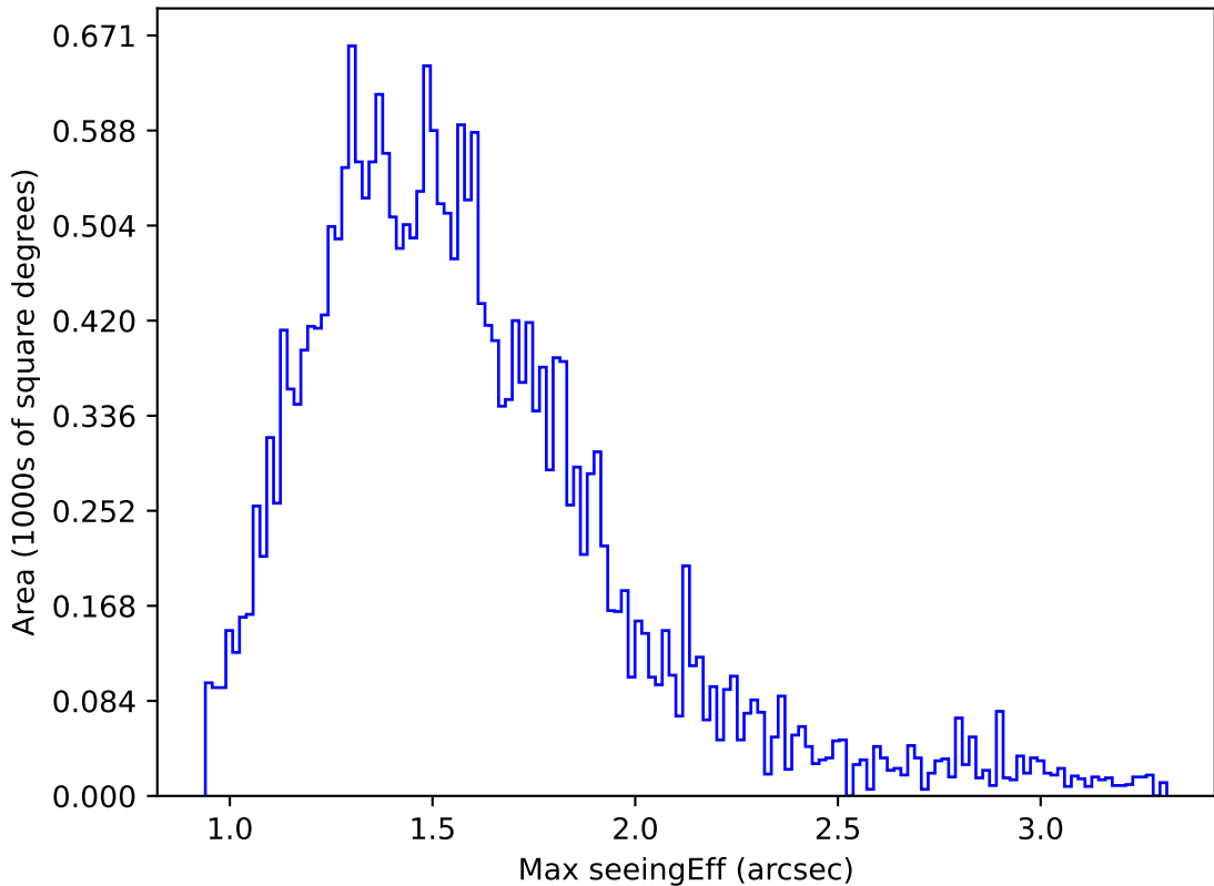
early_ss_template_fpextra2.0_v3.4_10yrs Yr 1 z band: Max seeingEff
