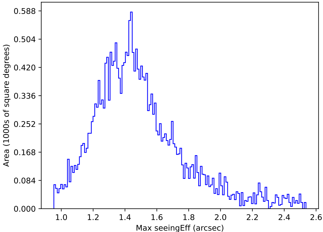
early_ss_template_fpextra2.0_v3.4_10yrs Yr 1 y band: Max seeingEff
