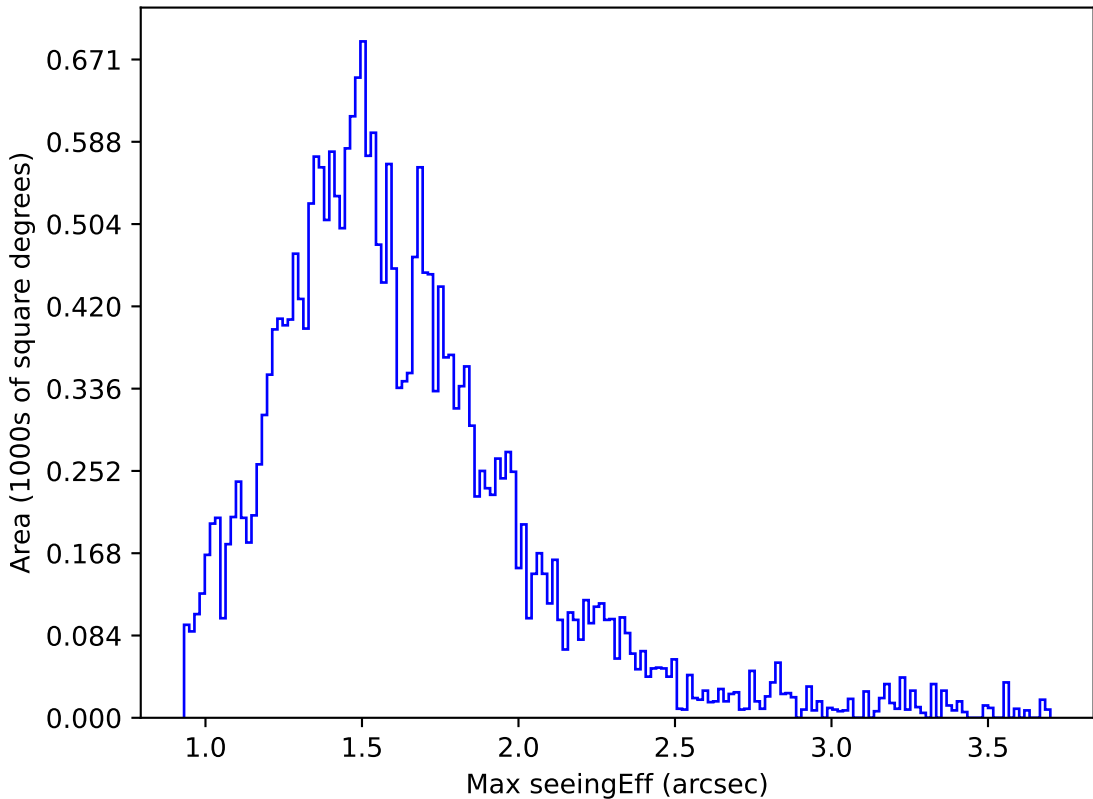
early_ss_template_fpextra2.0_v3.4_10yrs Yr 1 r band: Max seeingEff
