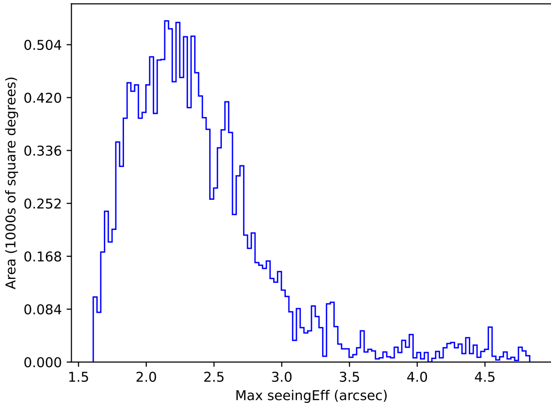
early_ss_template_fpextra2.0_v3.4_10yrs WFD y band: Max seeingEff
