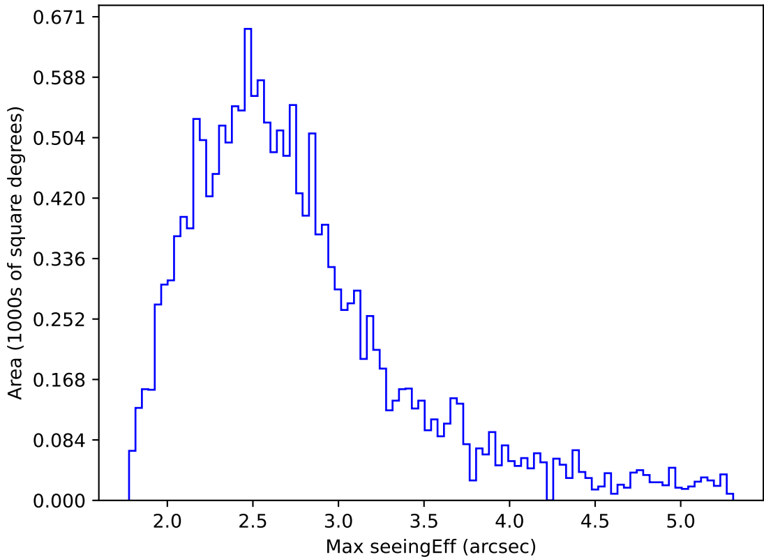
early_ss_template_fpextra2.0_v3.4_10yrs WFD i band: Max seeingEff
