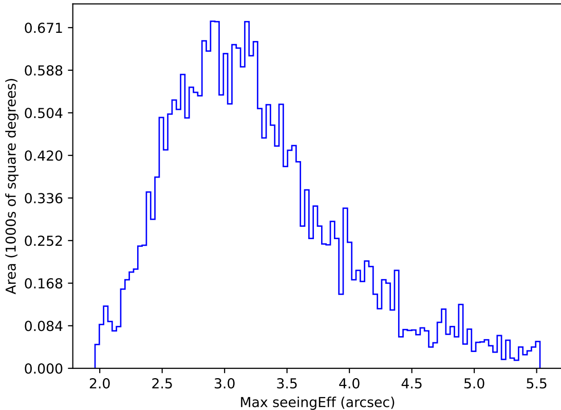
early_ss_template_fpextra2.0_v3.4_10yrs All sky all bands: Max seeingEff
