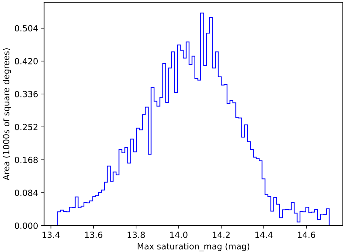
early_ss_template_fpextra2.0_v3.4_10yrs WFD u band: Max saturation_mag
