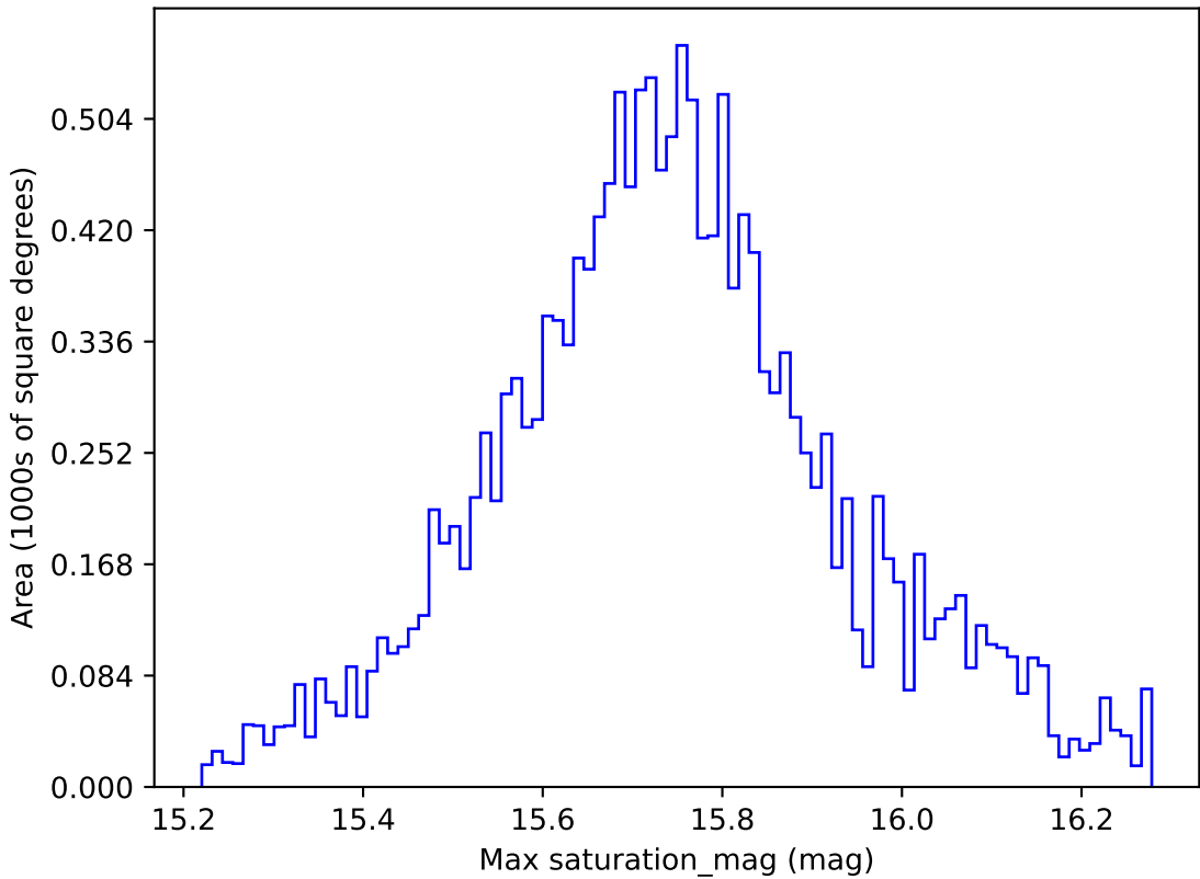
early_ss_template_fpextra2.0_v3.4_10yrs WFD g band: Max saturation_mag
