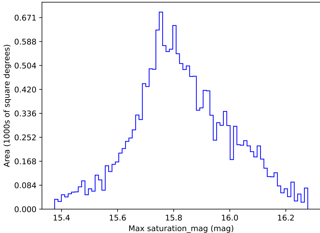
early_ss_template_fpextra2.0_v3.4_10yrs WFD all bands: Max saturation_mag
