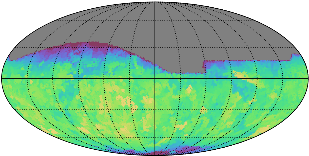
early_ss_template_fpextra2.0_v3.4_10yrs All sky i band: Max saturation_mag
