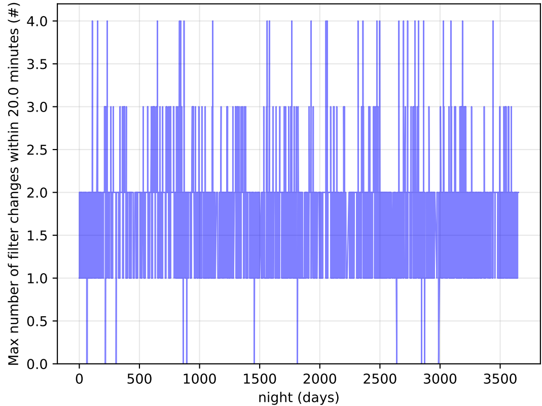
early_ss_template_fpextra2.0_v3.4_10yrs Per Night: Max number of filter changes within 20.0 minutes
