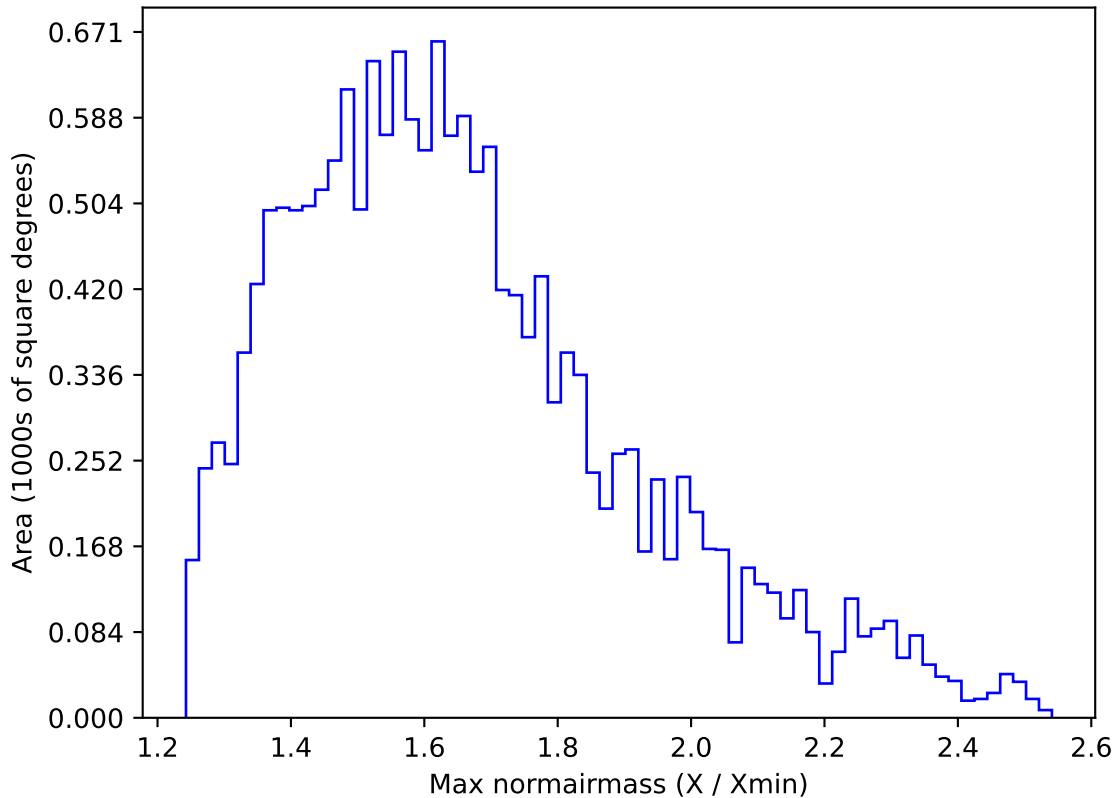
early_ss_template_fpextra2.0_v3.4_10yrs WFD u band: Max normairmass
