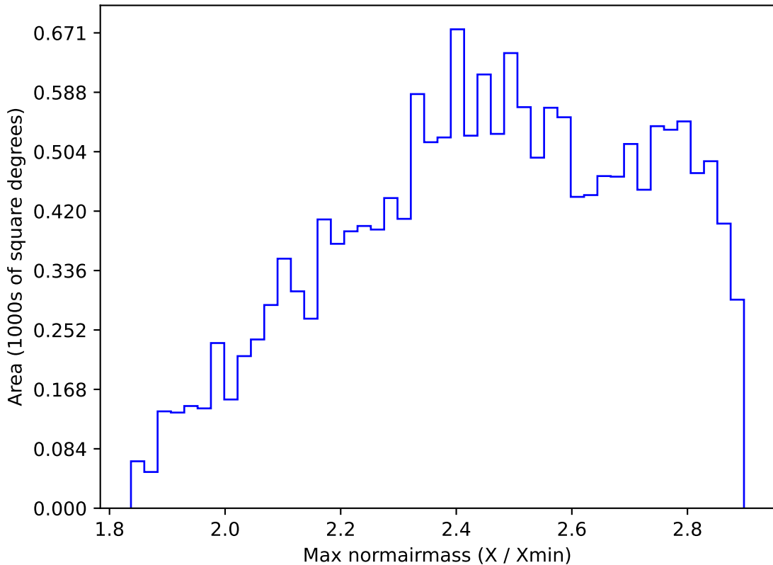
early_ss_template_fpextra2.0_v3.4_10yrs WFD all bands: Max normairmass
